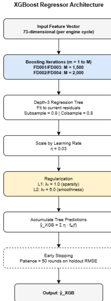
Figure 3.3 XGBoost architecture.
