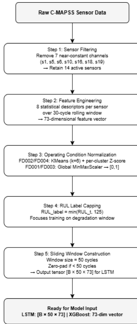
Figure 3.5 Preprocessing pipeline
